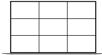
1500.960 (=920+920+920) 2064 x 1290 x 444
